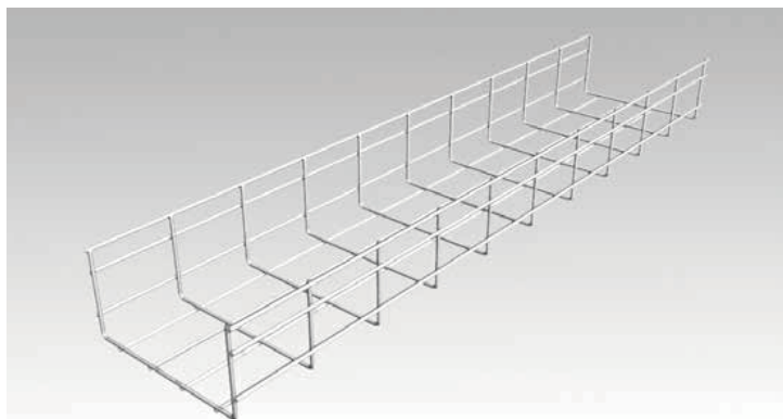
H100 R4 Wire Mesh Cable Tray SWL per 1.5m span
